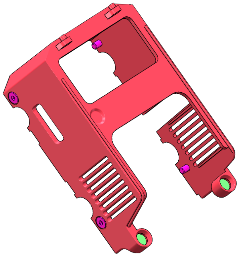
20.205.0123 挤出头外壳组件 Extruder Housing Assembly
