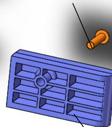
09.202.0060 内六角半圆头螺钉 M3*12 M3 x 12 Hex Socket Screw, Half Round Head
